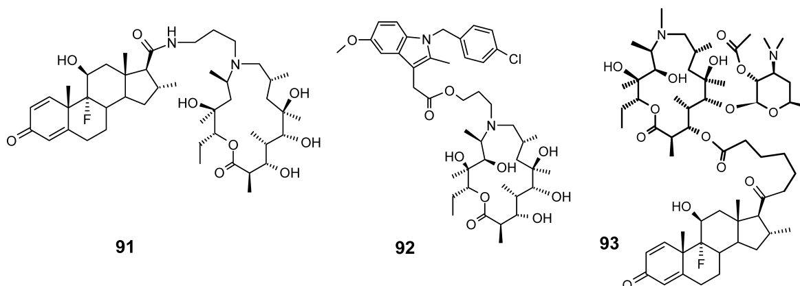
Fig. 23 Structures of complex 9a, N -substituted-aglycone and 3-substituted descladinosyl azalides.
