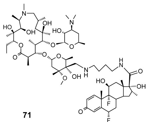
Fig. 16 Structure of potential anti-inflammatory 4''-C-tetramethylethylendiamino-steroido-substituted azalide.
