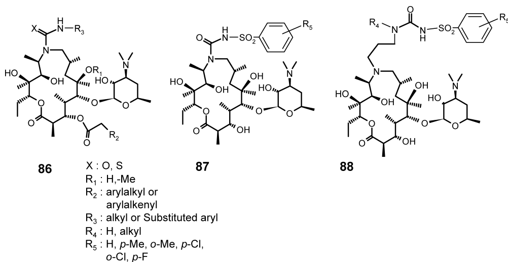
Fig. 21 Structures of 3-descladinosyl- N -carbamoyl derivatives of 9-deoxo-9-dihydro-9a-aza-homoerythromycin.
