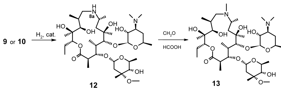
Scheme 5 Synthesis of 9-dihydro-9-deoxy-8a-methyl-8a-aza-8a-homoerythromycin ( 13 ).
